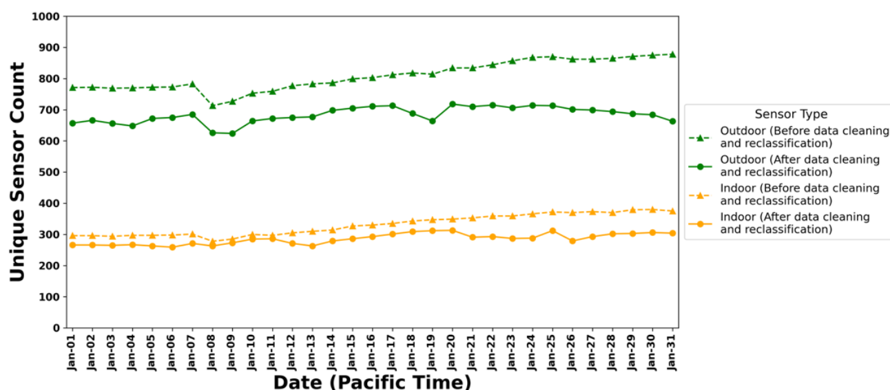
Figure 1. Daily count of unique indoor and outdoor activated PurpleAir sensors operating in the South Coast Air Basin (SCAB) during January 2025. Solid lines with circle markers represent sensors retained after data cleaning and reclassification, while dashed lines with triangle markers show counts before data cleaning and reclassification. Daily counts only include sensors recording at least 18 hours of data on a given day in Pacific Standard Time (PST).
