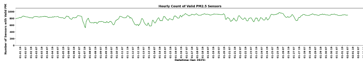
Figure S6. Hourly time series showing the number of PurpleAir sensors with valid PM 2.5 data across the South Coast Air Basin (SCAB) from January 1 to February 1, 2025. A sensor was considered valid for a given hour if it reported a non-missing pm2.5_atm_a measurement.
