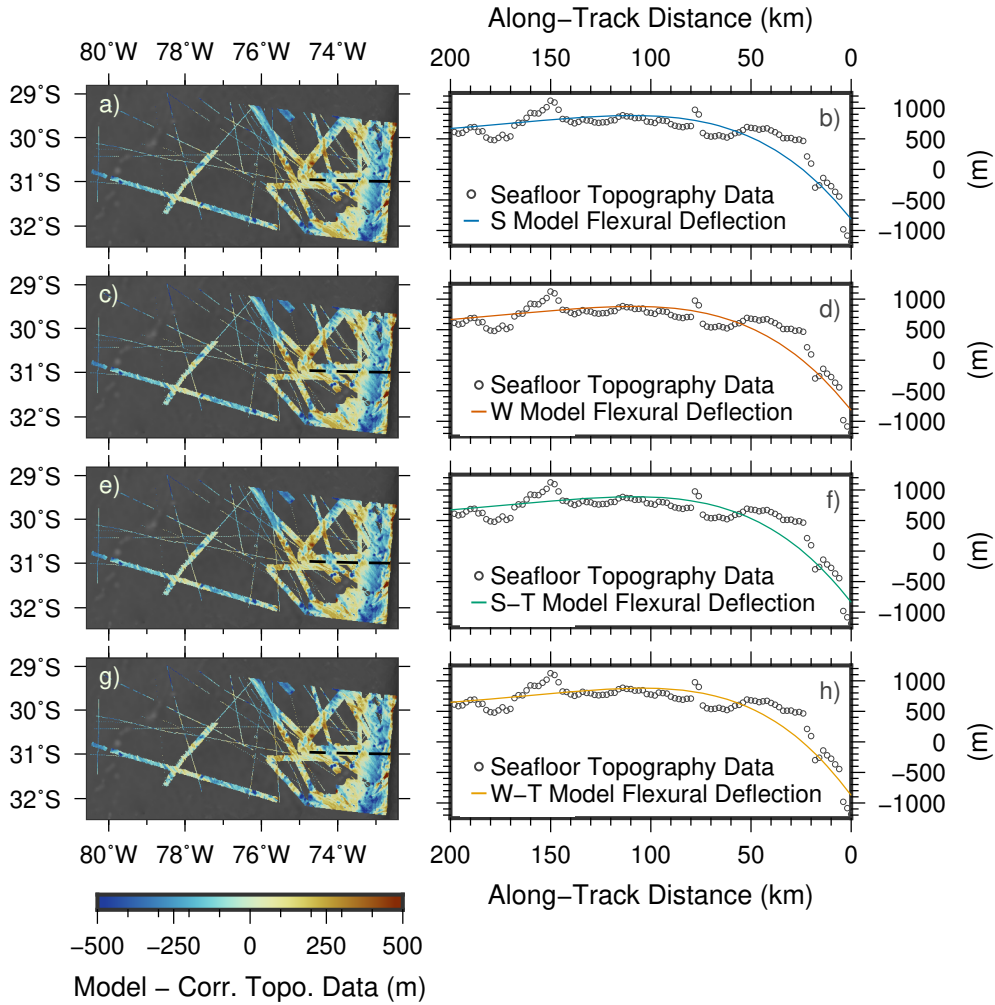
Figure 7. For a region offshore central Chile (ID: CL03), the residuals between the model flexural deflection and the seafloor topography data are shown for four different model setups depending on the value of the coefficient of friction and whether the effect of thermal stress was included (see text). Profiles of model fits for each case are also shown, with points for the data and a solid line for the model result. The sampling track is displayed as a dashed line in each map.
