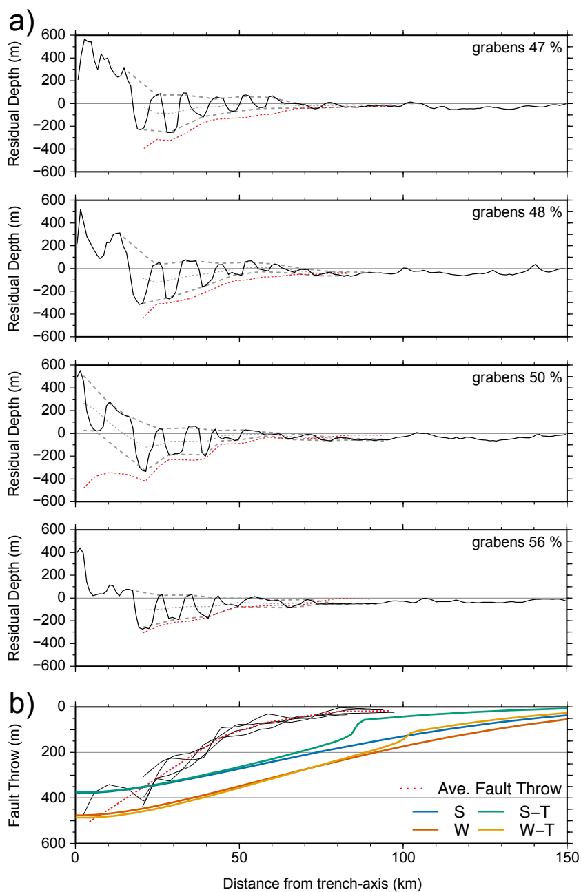
Figure 13. a) Profiles showing outer rise fractures in NE Japan between 39.5^{\circ} N and 40^{\circ} N. Figure nomenclature as in Fig. 12a. b) Stack of graben depths along-strike showing how the throw on normal faults increases toward the trench-axis. Dashed red line shows the average of these profiles. The estimated fault throws for the various sets of models are also plotted.
