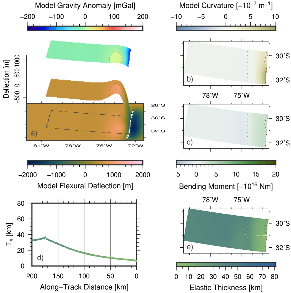
Figure 9. For a region offshore central Chile (ID:CL03) and using the W lithosphere rheology, a map of the original model output for the deflection w and a 3-D visualization of the best-fit flexural surface selected are shown in a). Also displayed in a) is the expected marine gravity anomaly \Delta g as calculated from w . The contours are drawn every 750 m for w and every 150 mGal for \Delta g . From w , the curvature as seen in b) is computed. The red dotted line marks the locations of the largest magnitudes of the curvature at the trench outer slope, while the blue dotted line traces the smallest magnitudes of the curvature just seaward of the outer rise. In turn, the curvature is used to compute the bending moment as seen in c). The elastic thickness values T_e are then obtained from the moment-curvature relation which is specific to the W set of models. Subfigure d) shows a trench-perpendicular profile of T_e , the location of which is shown in relation to the model region mapped in subfigure e).
