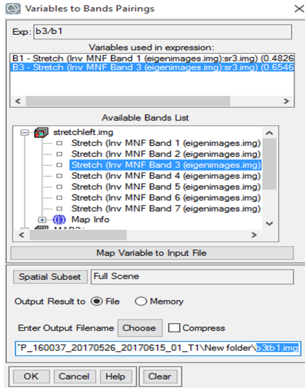
(Fig 3.4.1) using formula " b3/b1 " and saving it as "b3tb1.img"
