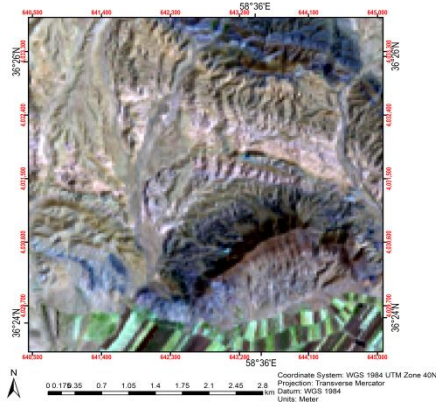
(Fig 4.3.6) The image "fe2.img" constructed from (MAP1, MAP11) by the Author with the name Fe mine in North West of Neyshabur city, Razavi Khorasan Province, Iran. ESM_4.3.2 original data available in Online Resource
