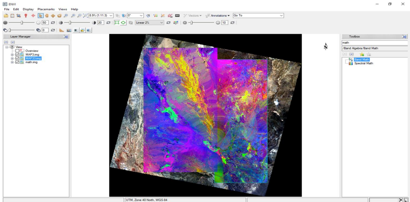
(Fig 3.4.4) "MAP3.img" and "MAP33.img"
