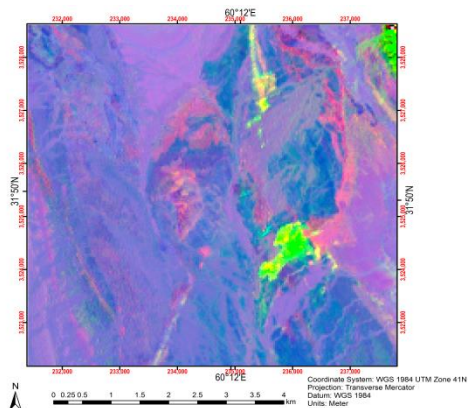
(Fig 4.5.4) The image "mg1111.img" constructed from (MAP4, MAP44) by the Author with the name Magnesium mine in Southeast of Sarbisheh city, South Khorasan province, Iran. ESM_4.5 original data available in Online Resource
