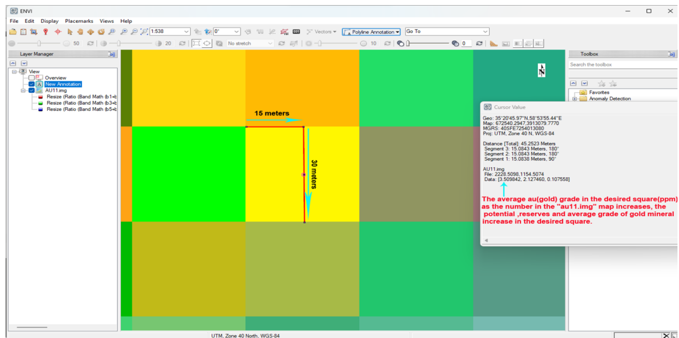
(Fig 4.1.4) The average of Gold (AU) grade (ppm) in the desired square (from the center of the square to a distance of fifteen meters around) shown by arrows in "AU11.img" map
