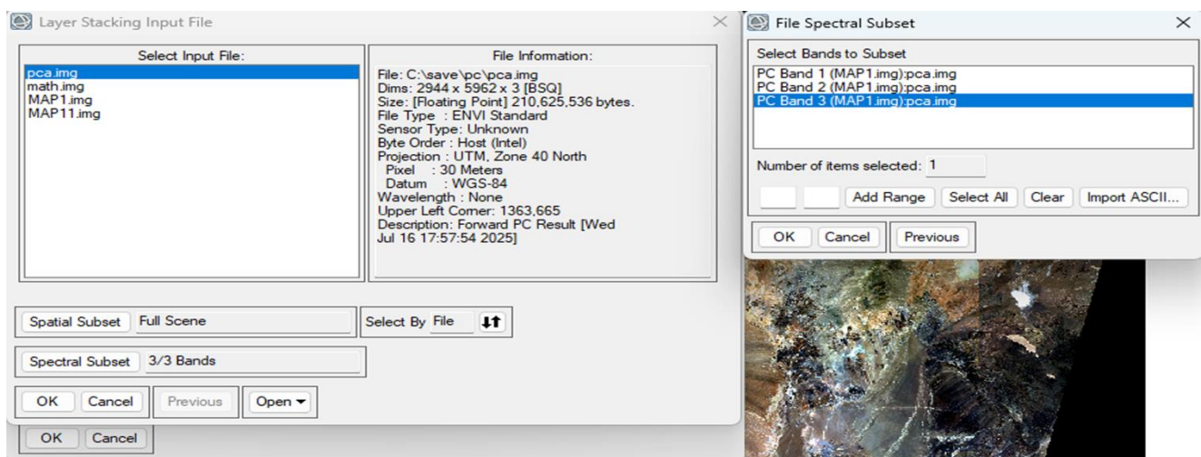
(Fig 3.5.2) selecting band 3 from "pca.img"
