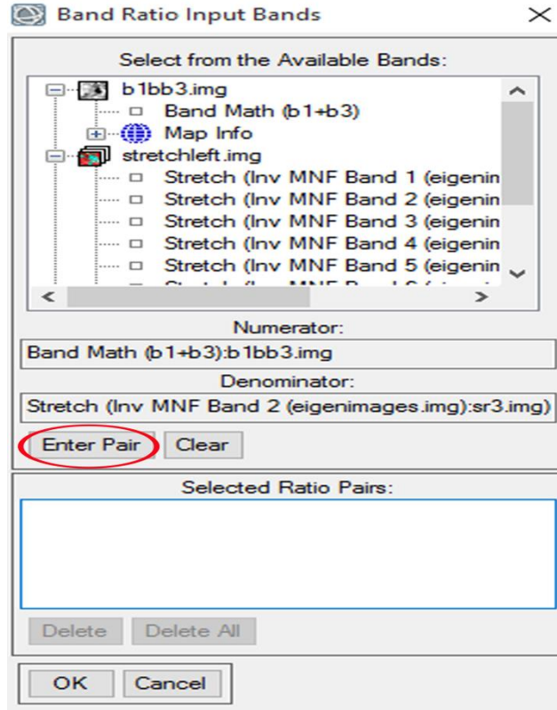
(Fig 3.3.4) using formula " ((b3+b1)/b2) "
