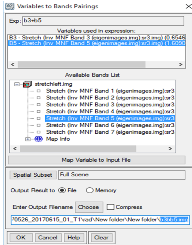
(Fig 3.3.2) applying formula "b3+b5" on "stretchleft.img" and saving it as "b3bb5.img"
