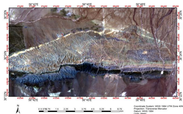
(Fig 4.6.1) The image "cr1.img" constructed from (MAP1, MAP11) by the Author with the name Chromite mine in west of Sabzevar city, Razavi Khorasan province, Iran. ESM_4.6 original data available in Online Resource
