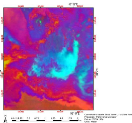
(Fig 4.3.4) The image "fe1111.img" constructed from (MAP4, MAP44) by the Author with the name Fe mine in the north of bam city, Kerman province, Iran. ESM_4.3.1 original data available in Online Resource
