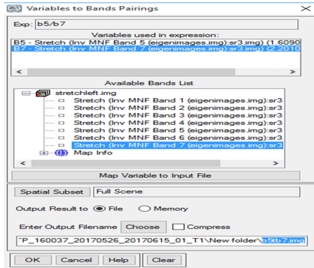
(Fig 3.4.2) using formula "(b5/b7)" and saving it as "b5tb7.img"
