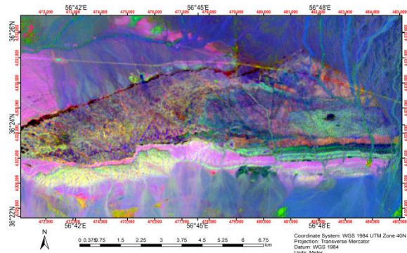
(Fig 4.6.4) The image "cr1111.img" constructed from (MAP4, MAP44) by the Author with the name Chromite mine in west of Sabzevar city, Razavi Khorasan province, Iran. ESM_4.6 original data available in Online Resource
