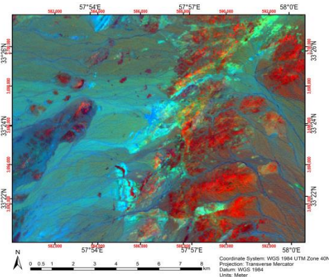
(Fig 4.9.2) The image "Industrial soil11.img" constructed from (MAP2, MAP22) by the Author with the name Industrial soil mine in Southeast of Boshruyeh city, South Khorasan province, Iran. ESM_4.9 original data available in Online Resource
