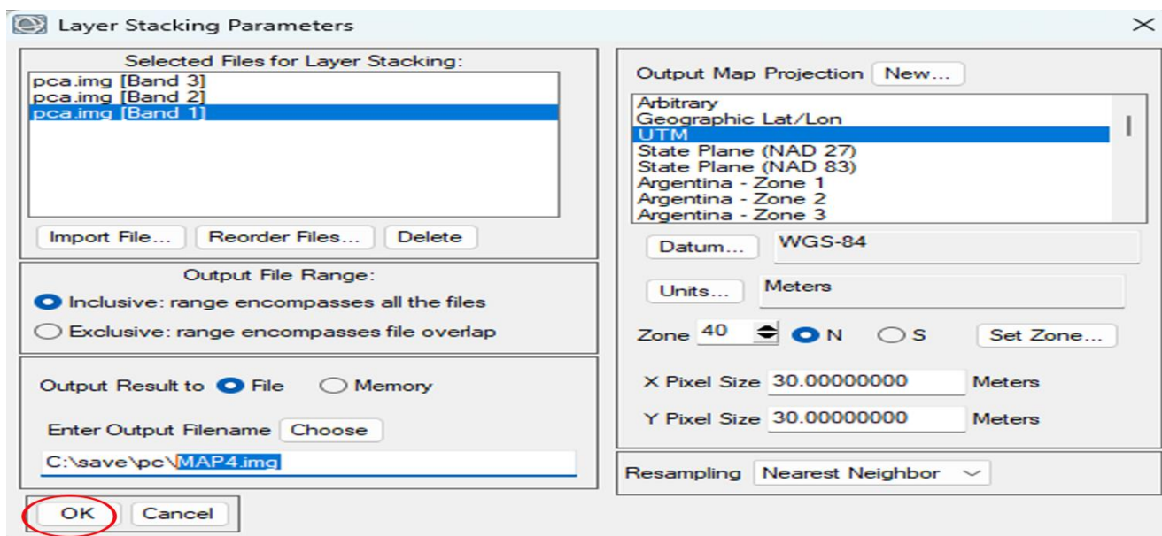
(Fig 3.5.3) stacking band compound (pca3, pca2, pca1) as RGB and saving it as "MAP4.img"
