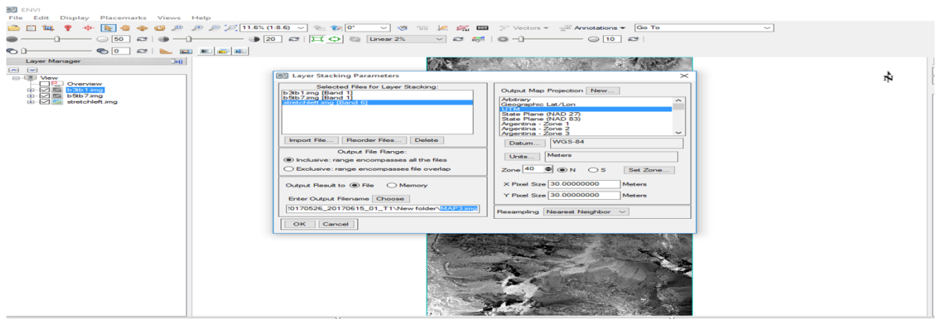
(Fig 3.4.3) stacking band compound ((b3/b1),(b5/b7),b6) as RGB and saving it as "MAP3.img"
