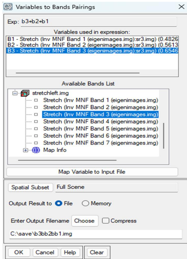
(Fig 3.2.3) applying formula "b3+b2+b1" on "stretchleft.img" and saving it as "b3bb2bb1.img"
