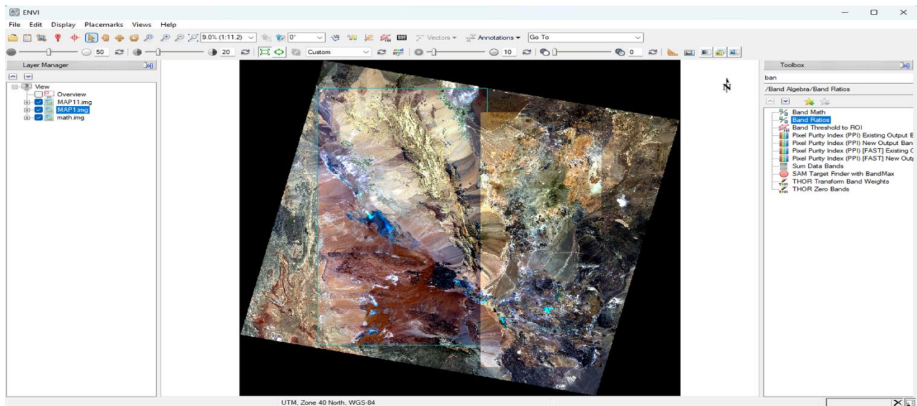
(Fig 3.2.8) "MAP1.img" and "MAP11.img"
