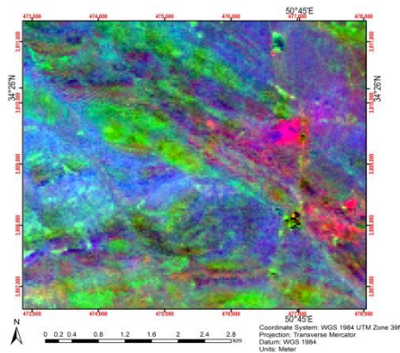
(Fig 4.4.3) The image "mn111.img" constructed from (MAP3, MAP33) by the Author with the name Manganese mine in Southwest of Qom city, Iran. ESM_4.4 original data available in Online Resource
