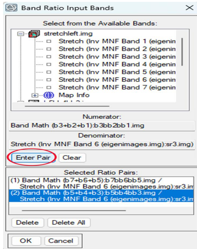
(Fig 3.2.6) using formula " ((b3+b2+b1)/b6) "
