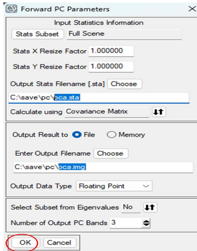
(Fig 3.5.1) saving "pca.img"
