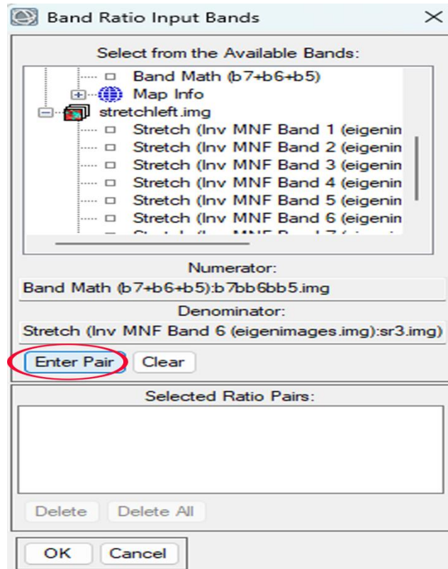
(Fig 3.2.4) using formula " ((b7+b6+b5)/b6) "
