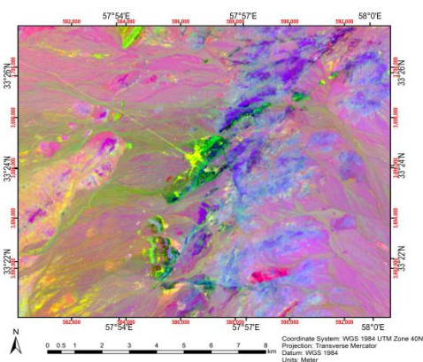
(Fig 4.9.4) The image "Industrial soil1111.img" constructed from (MAP4, MAP44) by the Author with the name Industrial soil mine in Southeast of Boshruyeh city, South Khorasan province, Iran. ESM_4.9 original data available in Online Resource
