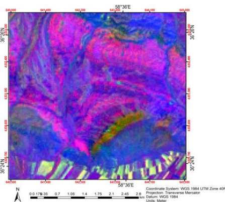
(Fig 4.3.8) The image "fe222.img" constructed from (MAP3, MAP33) by the Author with name Fe mine in North West of Neyshabur city, Razavi Khorasan Province, Iran. ESM_4.3.2 original data available in Online Resource
