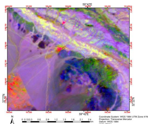
(Fig 4.11.4) The image "co1111.img" constructed from (MAP4, MAP44) by the Author with the name Cobalt mine in Southwest of Sarbisheh city, South Khorasan province, Iran. ESM_4.11 original data available in Online Resource
