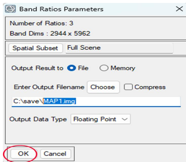
(Fig 3.2.7) saving "MAP1.img"
