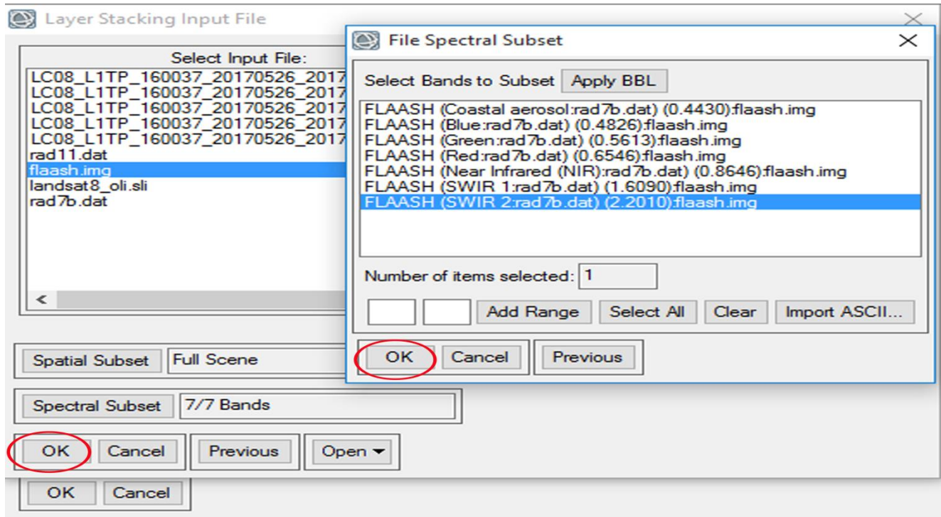
(Fig 2.3.3) selecting "SWIR 2" band from "Flaash.img"
