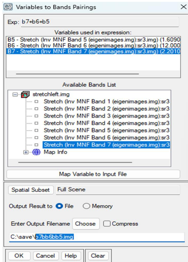
(Fig 3.2.1) applying formula "b7+b6+b5" on "stretchleft.img" and saving it as "b7bb6bb5.img"
