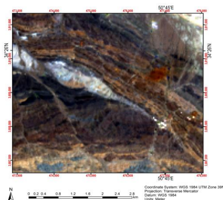
(Fig 4.4.1) The image "mn1.img" constructed from (MAP1, MAP11) by the Author with the name Manganese mine in Southwest of Qom city, Iran. ESM_4.4 original data available in Online Resource
