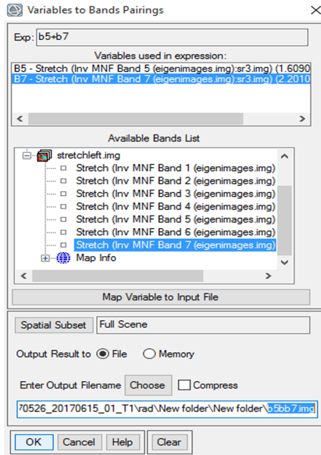
(Fig 3.3.3) applying formula “b5+b7” on “stretchleft.img” and saving it as “ b5bb7.img ”
