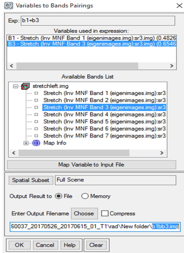
(Fig 3.3.1) applying formula "b1+b3" on "stretchleft.img" and saving it as "b1bb3.img"
