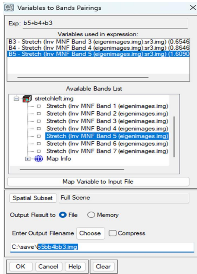
(Fig 3.2.2) applying formula "b5+b4+b3" on "stretchleft.img" and saving it as "b5bb4bb3.img"
