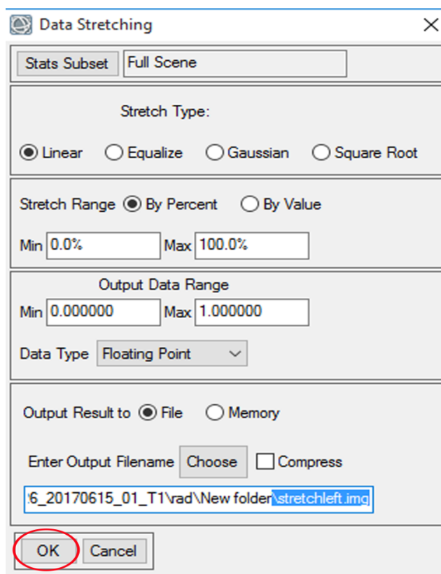
(Fig 3.5) "stretch" setting on "r3.img"
