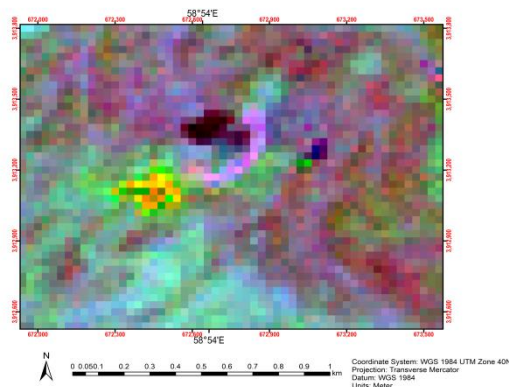
(Fig 4.1.2) The image "AU11.img" constructed from (MAP2, MAP22) by the Author with the name Iran Zarmehr mine. ESM_4.1 original data available in Online Resource
