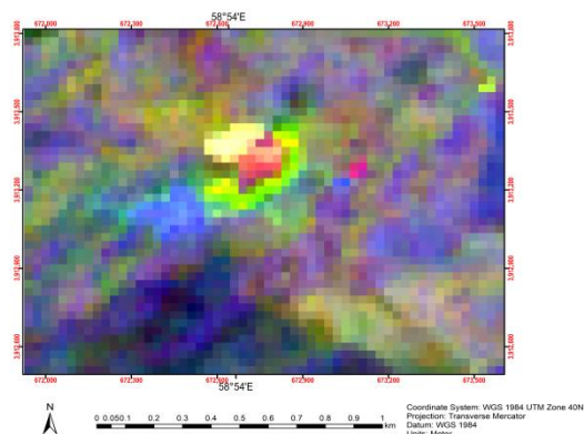
(Fig 4.1.4) The image "AU111.img" constructed from (MAP4, MAP44) by the Author with the name Iran zarmehr mine. ESM_4.1 original data available in Online Resource
