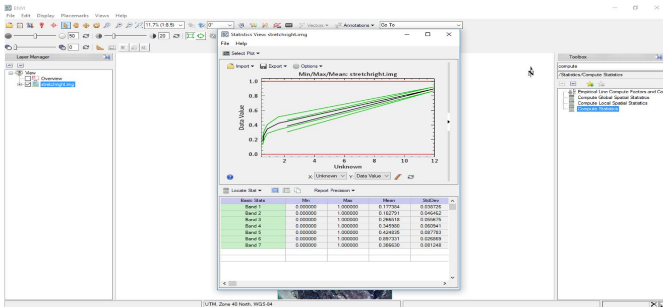
(Fig 3.1.4) Histogram stretched in "stretchright.img" while using thermal band11
