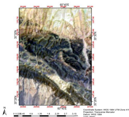
(Fig 4.12.1) The image "pb1.img" constructed from (MAP1, MAP11) by the Author with the name lead mine in North of Torbat-e Jam, Razavi Khorasan Province, Iran. ESM_4.12 original data available in Online Resource
