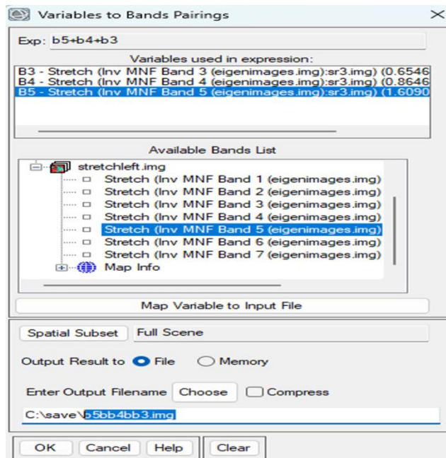
(Fig 3.2.2) applying formula "b5+b4+b3" on "stretchleft.img" and saving it as "b5bb4bb3.img"
