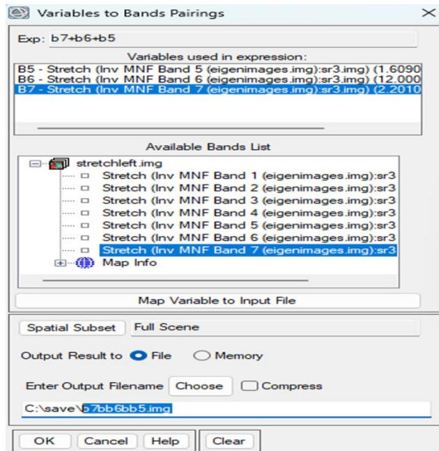
(Fig 3.2.1) applying formula "b7+b6+b5" on "stretchleft.img" and saving it as "b7bb6bb5.img"
