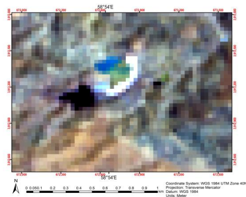
(Fig 4.1.1) The image "AU1.img" constructed from (MAP1, MAP11) by the Author with the name of Iran Zarmehr mine. ESM_4.1 original data available in Online Resource
