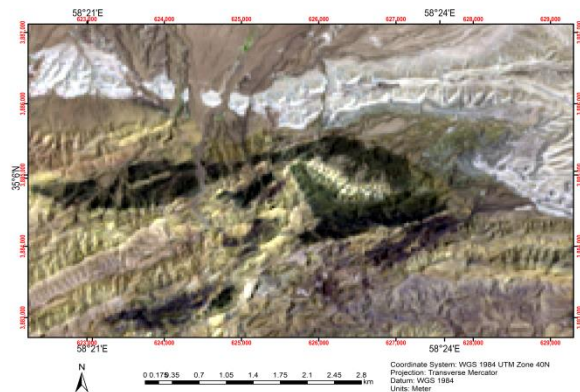
(Fig 4.2.1) The image "cu1.img" constructed from (MAP1, MAP11) by the Author with the name of Copper mine in Bardskan city, Razavi Khorasan Province, Iran. ESM_4.2 original data available in Online Resource
