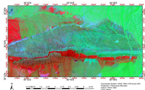
(Fig 4.6.2) The image "cr11.img" constructed from (MAP2, MAP22) by the Author with the name Chromite mine in west of Sabzevar city, Razavi Khorasan province, Iran. ESM_4.6 original data available in Online Resource
