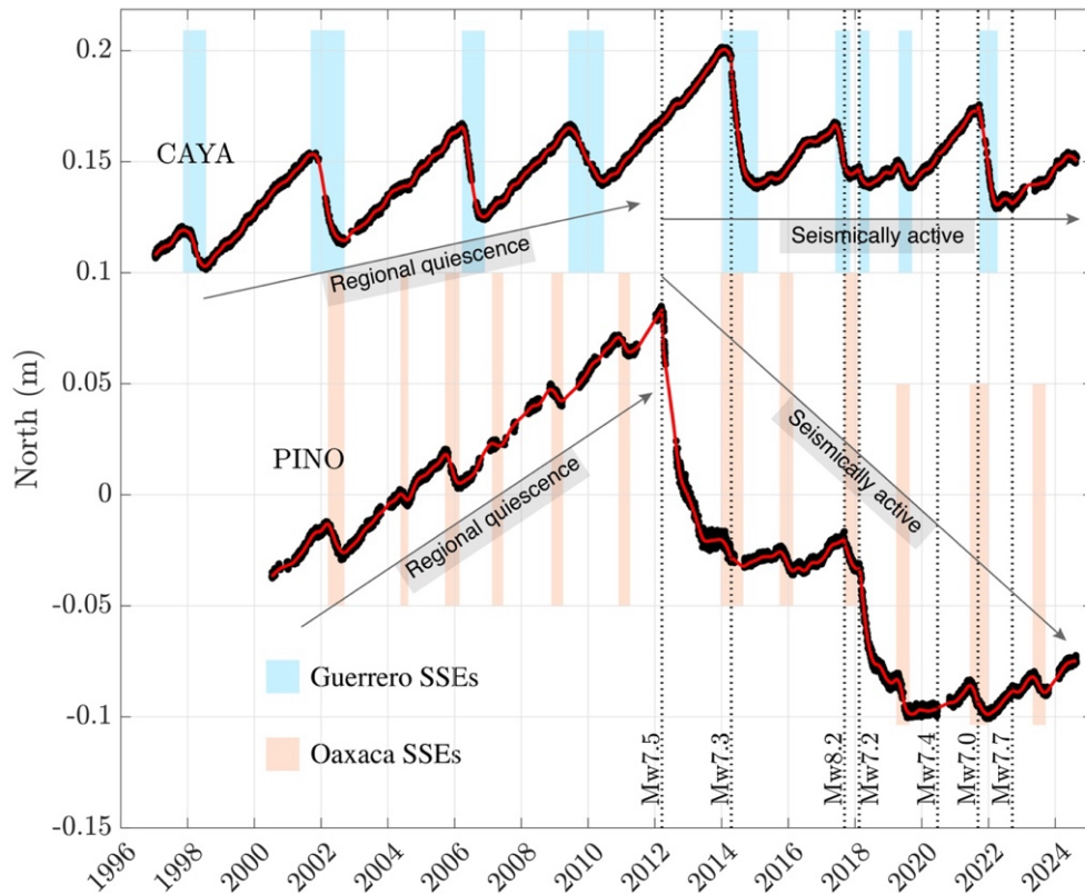
566 Figure 1 Long-term GPS record at two permanent stations in the states of Guerrero and Oaxaca 568 (see Figure 4 for stations location). Arrows indicate the effective strain rate during phases of regional seismic quiescence (left) and seismic activity (right). Dashed lines indicate the dates 570 of all M7+ earthquakes in the region. Light blue and orange rectangles indicate the periods of SSEs in Guerrero and Oaxaca, respectively.
