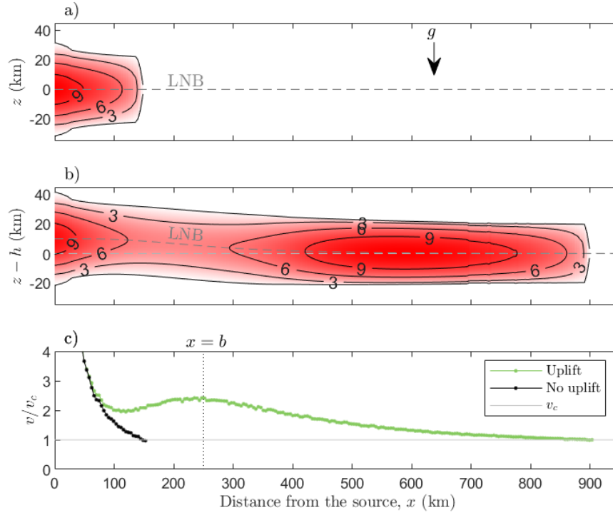
Figure A.1. Comparison of laterally propagating dyke shapes that include tip-blockage. This figure is a modified version of Figure 3, illustrating the impact of including blockage of the vertical dyke tips and centerline solid pressures as described in §2(e).iii & iv. The simulation properties are detailed in §3(a). This figure highlights the differences in dyke behaviour when the additional cross-sectional physical constraints are applied.
