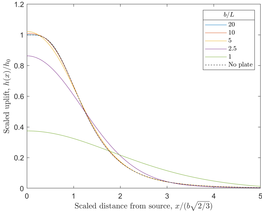
Fig. S3. Changes to the domal uplift profile as the bending length (S2) increases relative to the plume head radius. x is scaled by (S1) and h by (2.11).
