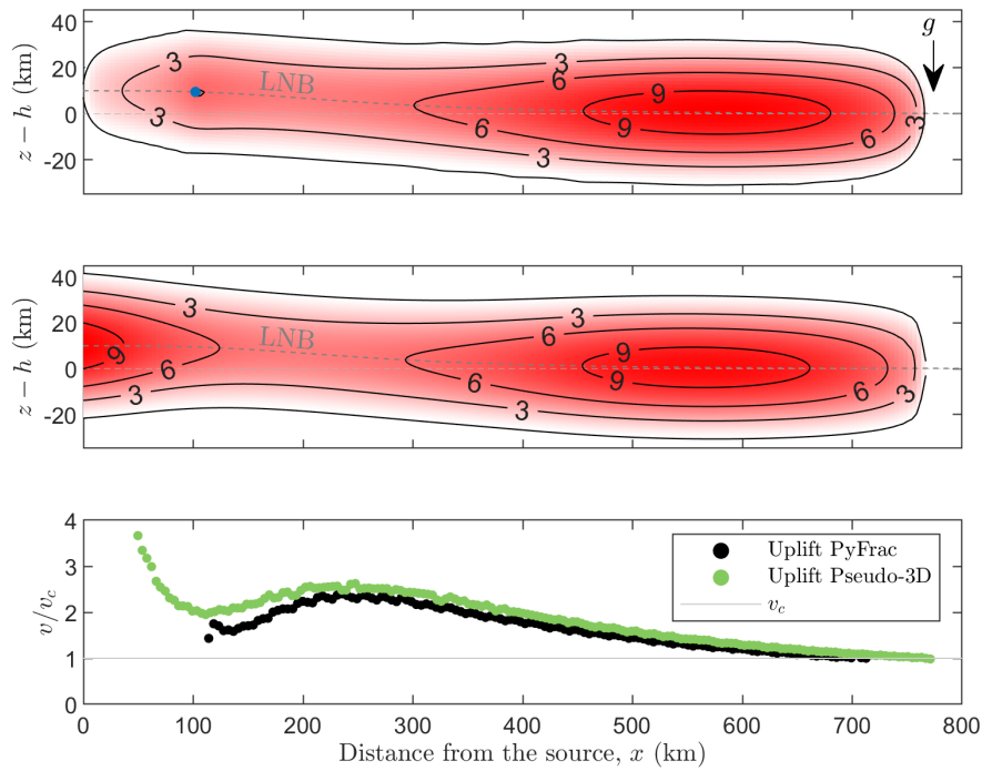
Fig. S1. A comparison of a fully 3D numerical simulator (PyFrac) to our pseudo-3D simulation of a laterally propagating dyke. Simulation properties are detailed in §3(a). Note the maximum LNB uplift h_0 is 1 km but has been exaggerated here to highlight its distortion. Panel a shows a simulation using the full 3D numerical simulator [60]. The dyke is driven by a volumetric flux Q from the blue dot with a value determined by (A 5). Panel b shows a corresponding simulation using our pseudo-3D model, with a pressure boundary at the source x = 0 . Panel c compares the lateral tip speeds of the two models.
