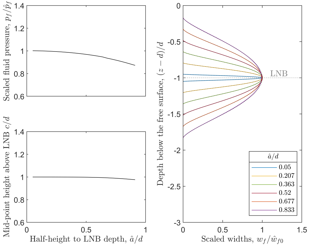
Fig. S1. Dykes in a crust of linearly increasing density, approaching the free surface. Panel a shows the fluid pressure ( p_f ). Panel b shows the width of the dyke hardly changes. In the y-axis the free surface is at zero and the LNB is at minus one; dashed black lines are the analytical full-space width \hat{w}_f . Panel c shows the minor offset of the dyke's centre above the LNB ( c ) such that the condition K_I(z = \pm a) = 0 is met.
