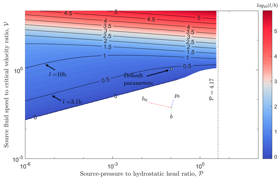
Figure B.1. ODE predictions of the final length of the dyke in the presence of domal uplift. Uplift is not strong enough to have an influence on length in the areas shown in white, thus in these areas the final dyke length tends to \hat{l} . To aid the interpretation of Figure 5, we indicate the directions travelled when h_0 , p_0 and b are increased are indicated.
