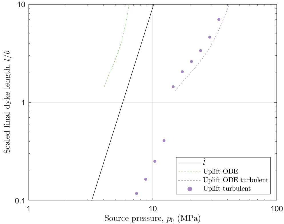
Fig. S2. Source pressure dependence vs dyke length, including the effect of turbulence. Note the increase in dyke length to that of the swell size, when the pressure is large enough, compared to the laminar case (Fig. 5).
