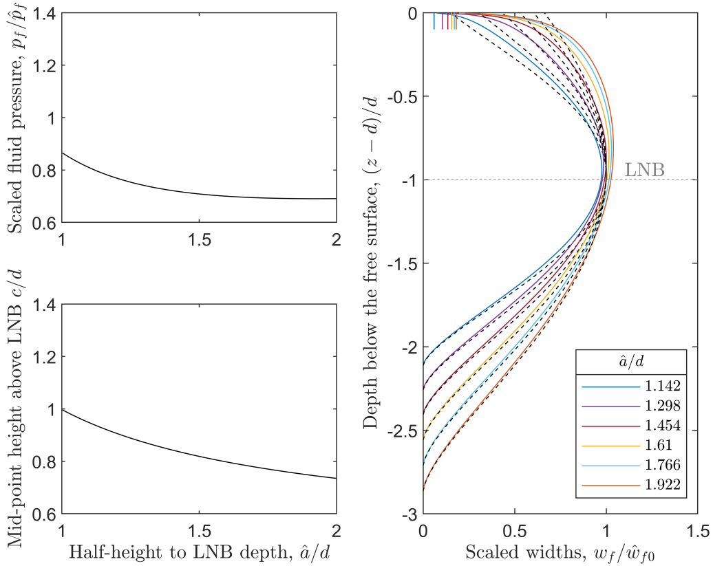
Fig. S2. This figure is a modified version of figure S1, showing dykes in a crust of linearly increasing density, that have breached the free surface. Panel b shows vertical lines which are the opening at the free surface. Here, dashed black lines are the analytical full-space width \hat{w}_f .
