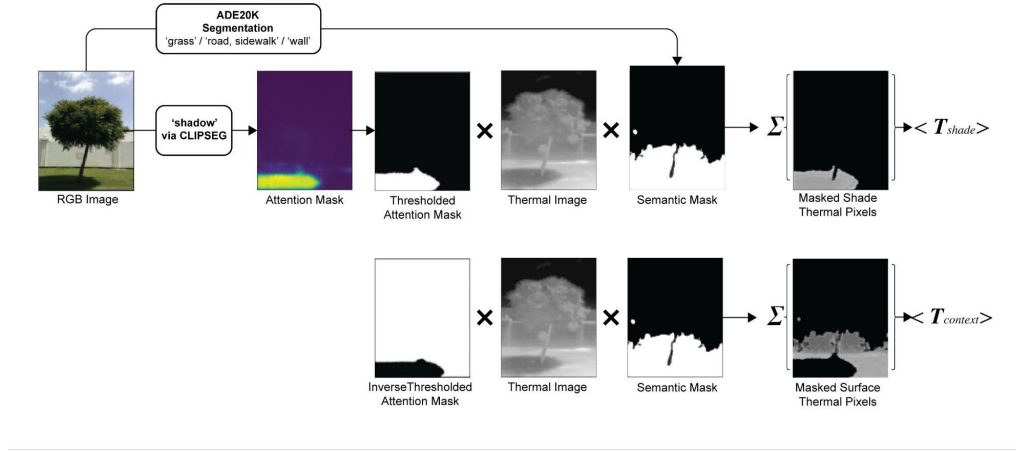
Figure 11: Segmentation of tree shadows
